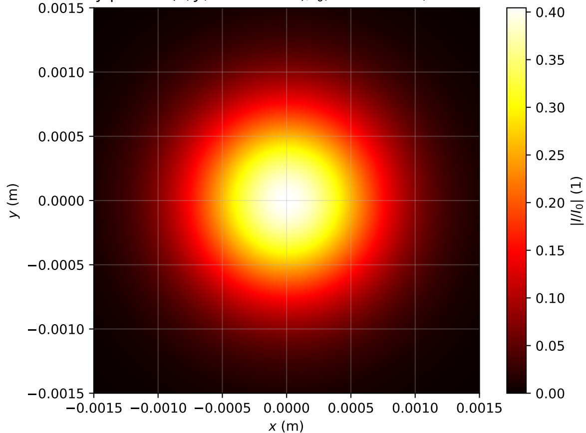
Intensity profile I(x, y, z = 3.105m)/I_0 , P_{in}=0.3P_{cr} , artificial time
